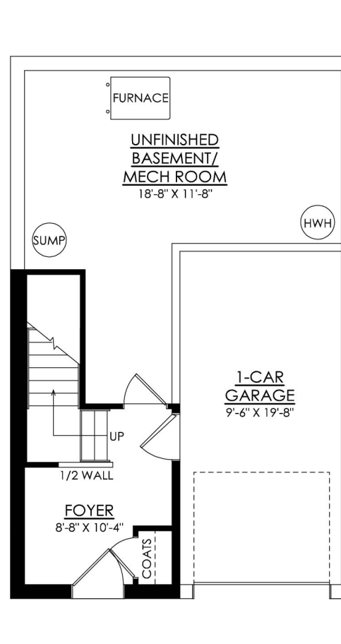
CITYLIGHTS- DESIGN 2 GROUND FLOOR TRADITIONAL & COUNTRY STARTING AT 1424 SF
